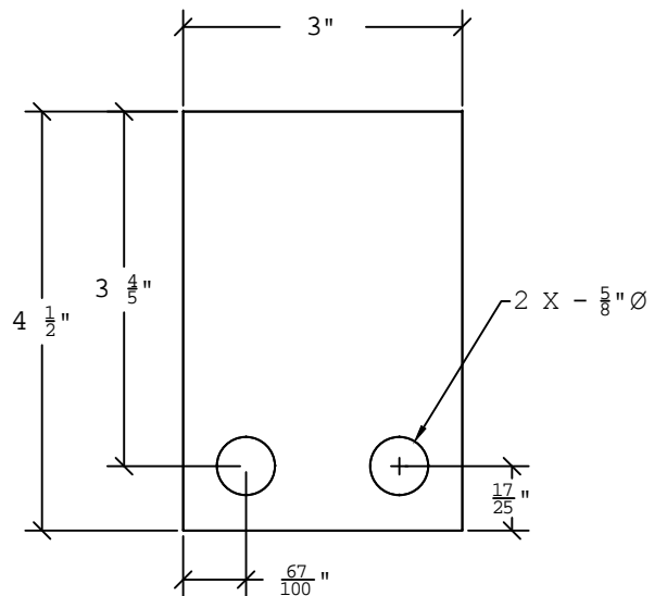
Top View of Footplate 10 Gage Steel (THK-.1345")
